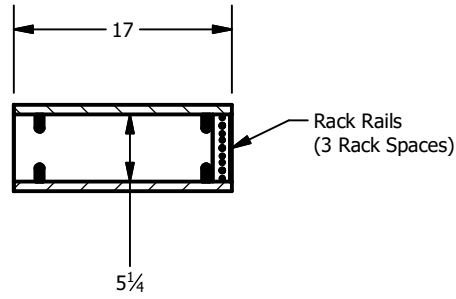
SECTION A-A SCALE 1 / 15
