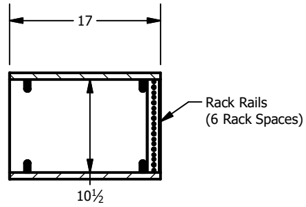
SECTION A-A SCALE 1 / 15
